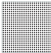
#17 Straight Open area 17.10% Centers 0.2012" Diameter 0.0938"
