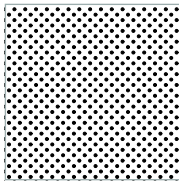
#23 Staggered Open area 23.0% Centers 0.160" Diameter 0.063"
