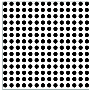
#29 Straight Open area 29.50% Centers 0.256" Diameter 0.157"
