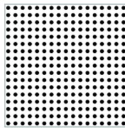
#16 Straight Open area 16.0% Centers 0.216" Diameter 0.098"
