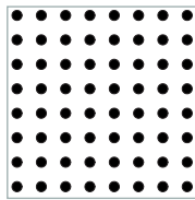
#13 Straight Open area 13.40% Centers 0.3789" Diameter 0.1562"
