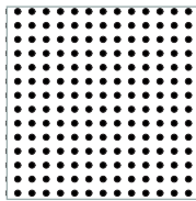
#14 Straight Open area 14.70% Centers 0.2706" Diameter 0.117"
