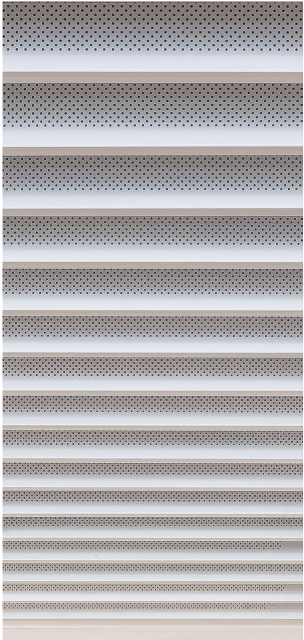
S06 Straight Diameter 0.125 Open area 19.6% Centers 0.25
