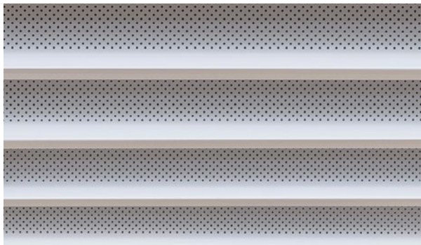
P19 Staggered Diameter 0.063 Open area 22.7% Centers 0.125
